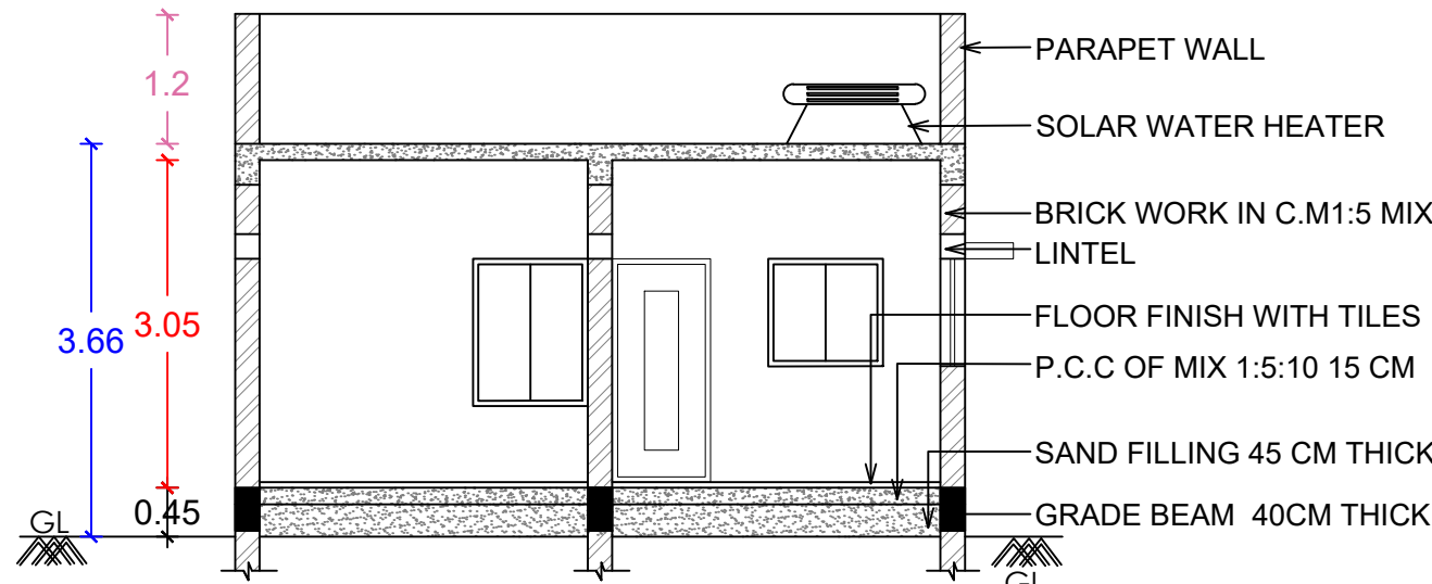
SECTION- AB
