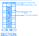
SECTION PLAN
