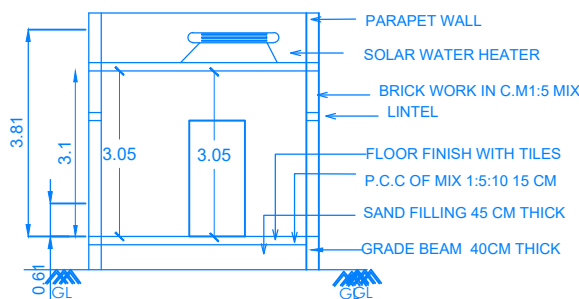
SECTION- AA1
