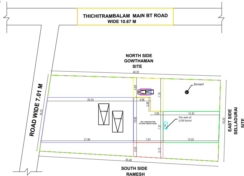
SITE PLAN
