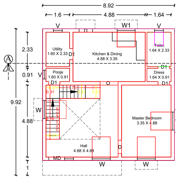
GROUND FLOOR PLAN BLOCK 1
