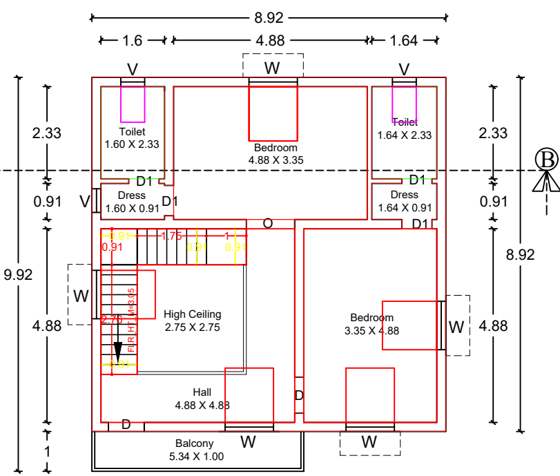
FIRST FLOOR PLAN BLOCK 2
