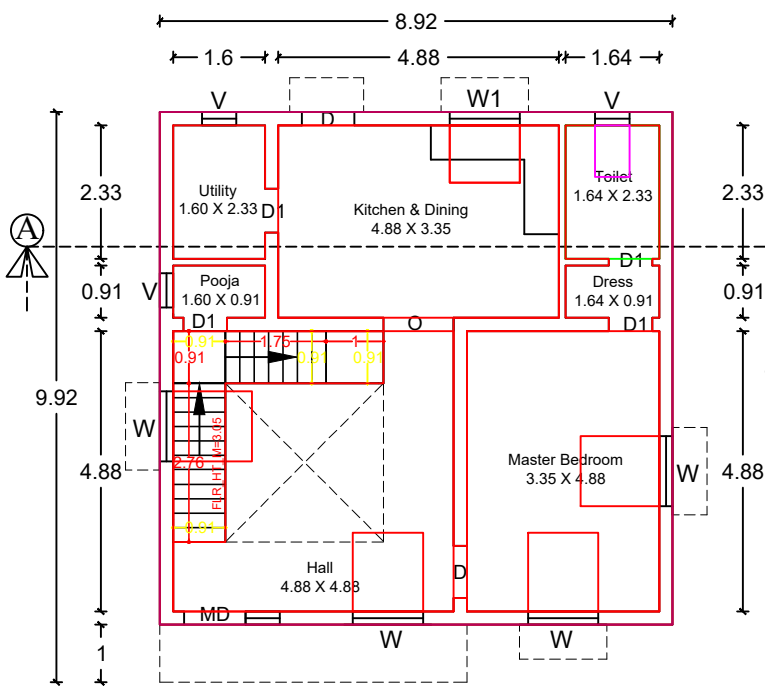
GROUND FLOOR PLAN BLOCK 2
