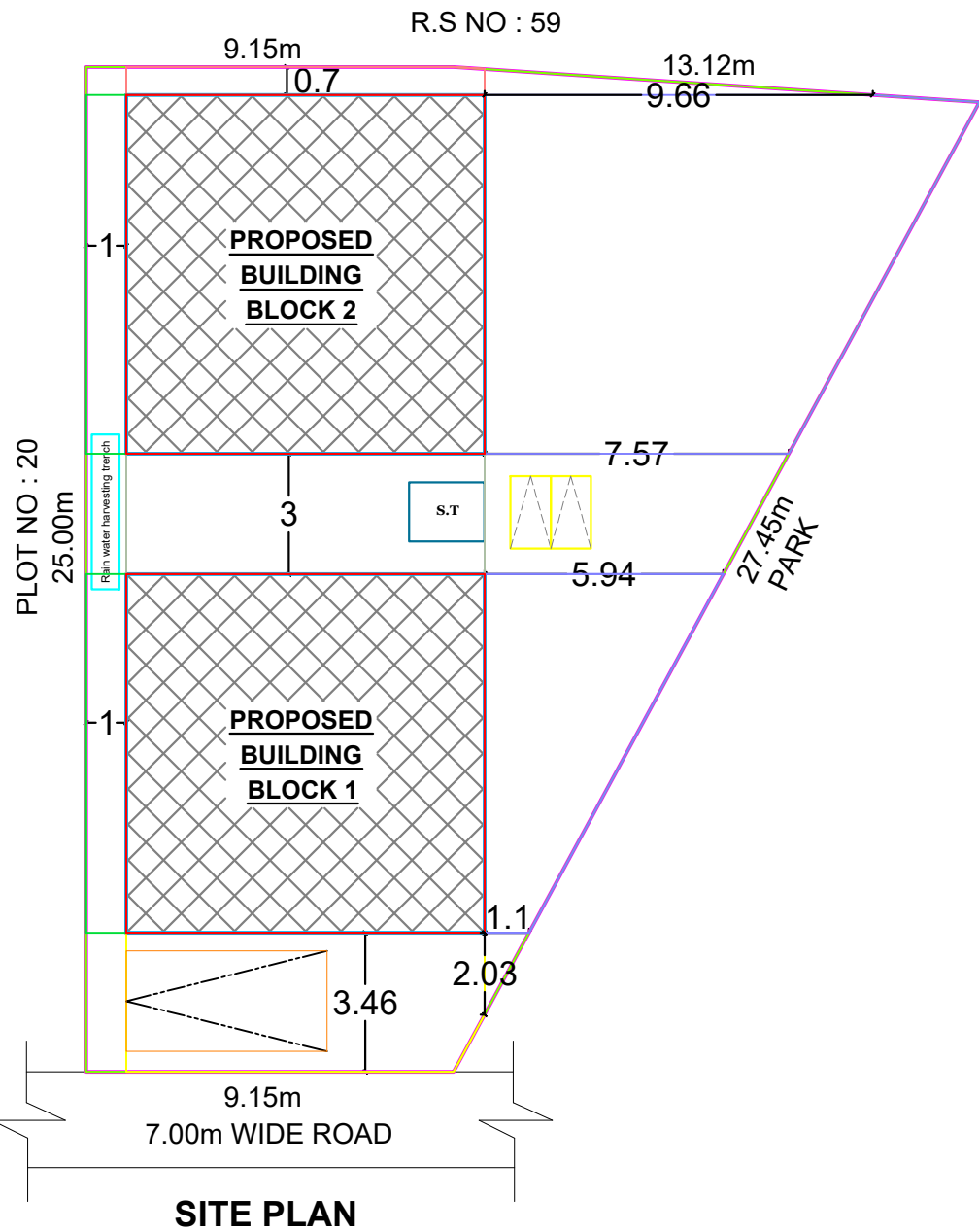
SITE PLAN
