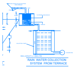
RAIN WATER COLLECTION SYSTEM FROM TERRACE
