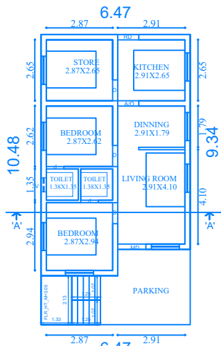
GROUND OR PLAN
