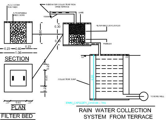
RAIN WATER COLLECTION SYSTEM FROM TERRACE
