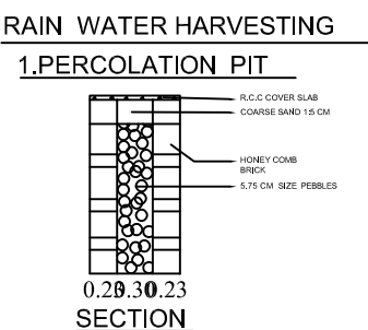
RAIN WATER HARVESTING 1. PERCOLATION PIT
