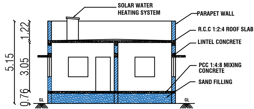
SECTION NO - "AB"
