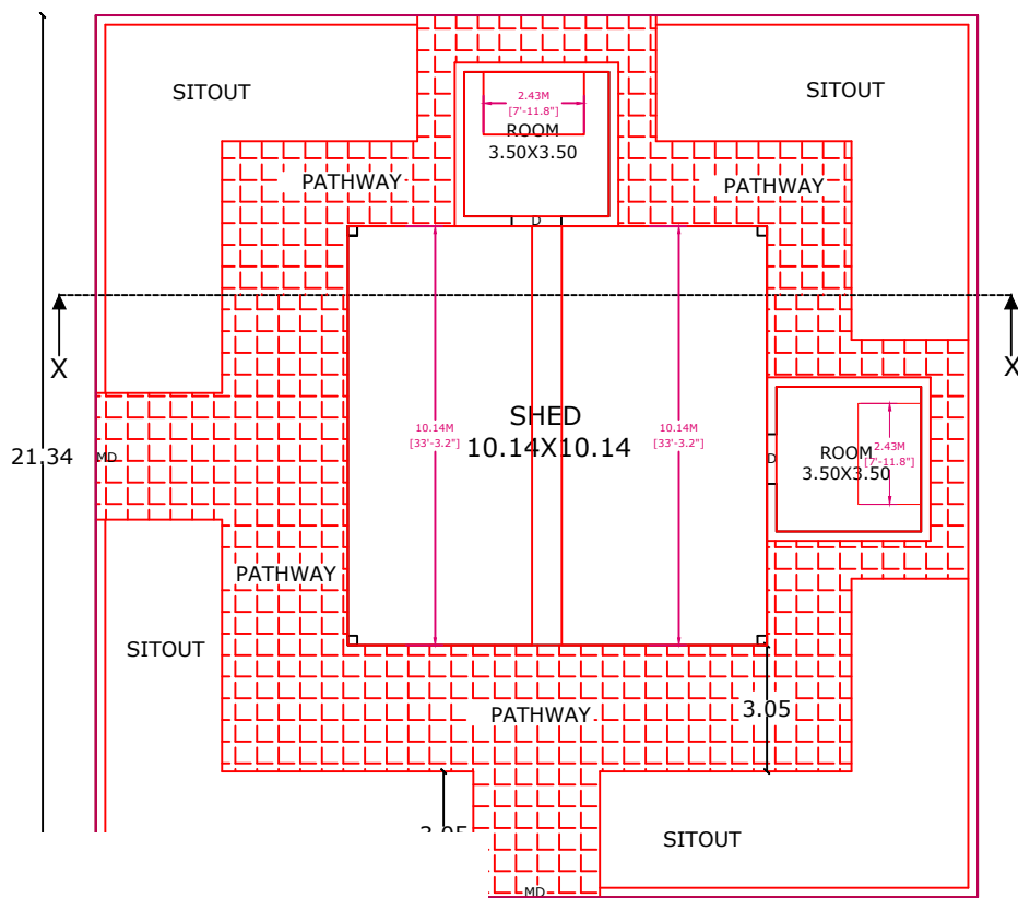
FLOOR PLAN
