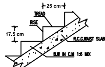
SECTION OF STAIRCASE
