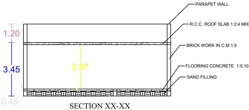
SECTION XX-XX
