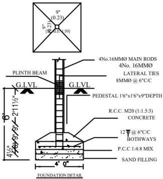
FOUNDATION DETAIL
