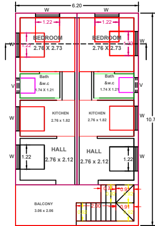
PRO. SECOND FLOOR
