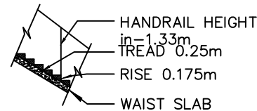
STAIRCASE DETAILS
