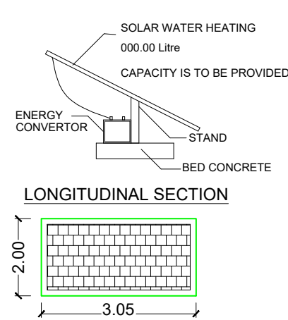
SOLAR SYSTEM
