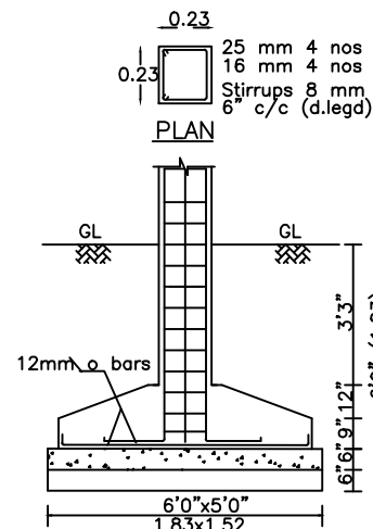
SECTION ON "A S"
