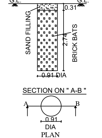
DETAILED PLAN OF RAINWATER PERCUSSION AND COLLECTION PIT
