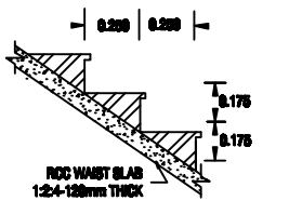
STAIR CASE STEPS
