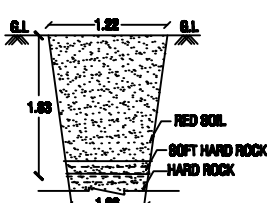
TRAIL PIT DETAIL
