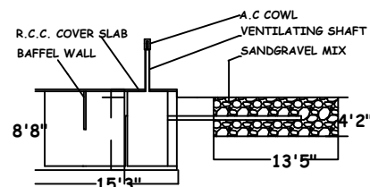
SEPTIC TANK AND DISPERSION TRENCH DETAILS
