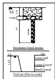
SEPTIC TANK AND DISPERSION TRENCH DETAILS
