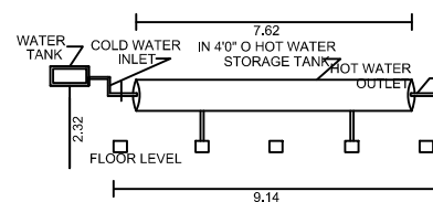
SOLAR HOT WATER SYSTEM DETAILS
