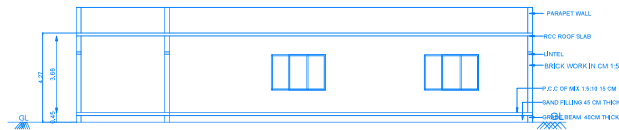
SECTION - AA1
