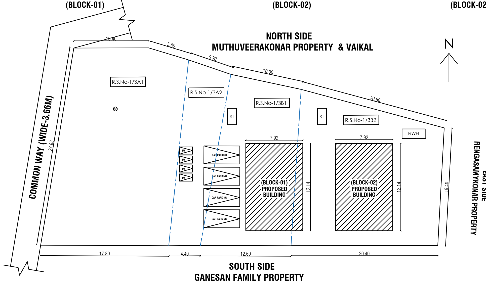
PRO.GROUND FLOOR PLAN (BLOCK-01)
