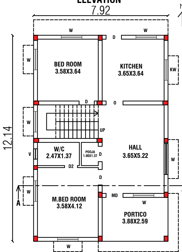
PRO.GROUND FLOOR PLAN (BLOCK-01)
