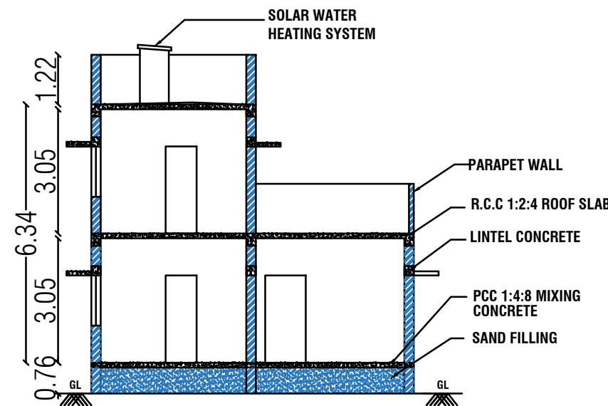
SECTION NO -"AB"
