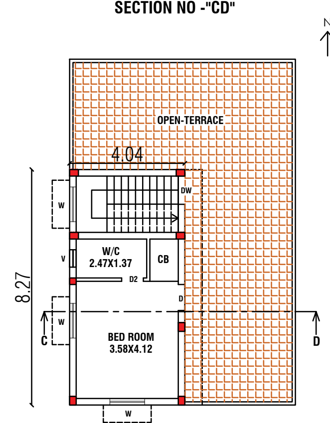
PRO.GROUND FLOOR PLAN (BLOCK-02)
