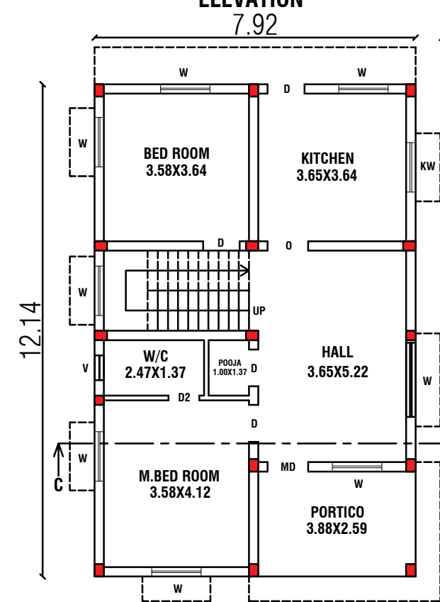
PRO.GROUND FLOOR PLAN (BLOCK-02)
