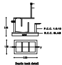
Septic tank detail
