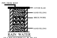
RAIN WATER HARVESTING R.W.H
