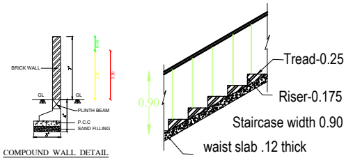
STAIR CASE DETAIL
