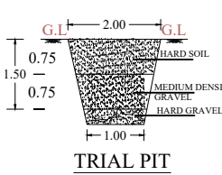
TRIAL PIT
