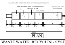
WASTE WATER RECYCLING SYSTEM
