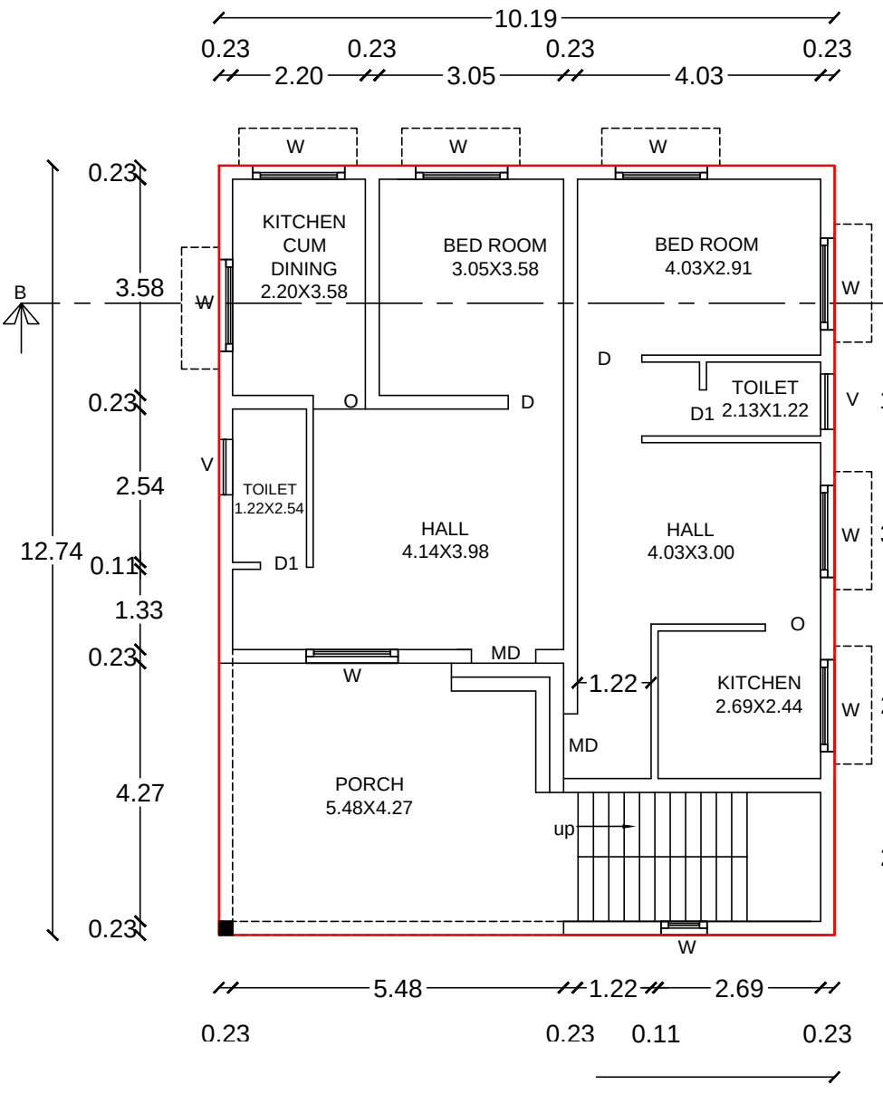
GROUND PLAN
