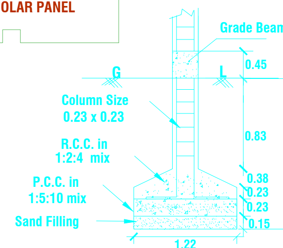
COLUMN DETAILS
