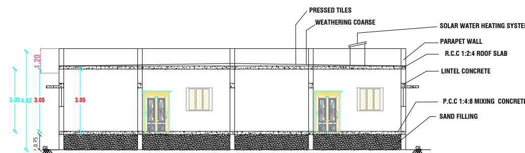
SECTION NO -"AA"
