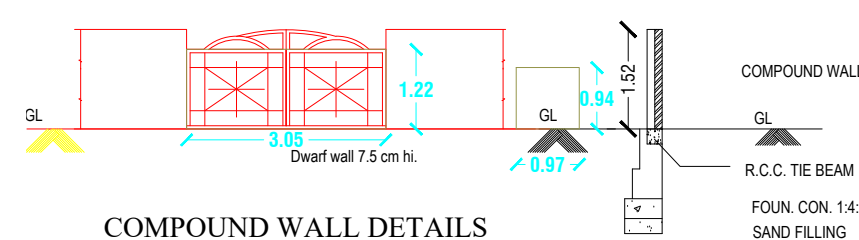
SECTION
