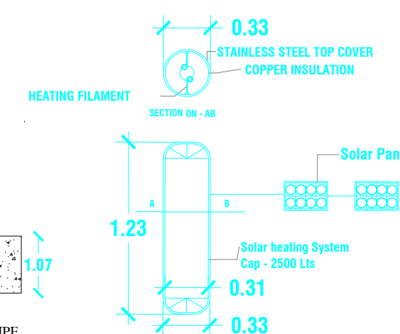
PLAN OF SOLAR WATER HEATING SYSTEM
