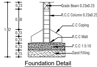
Foundation Detail
