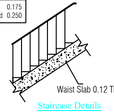
Staircase Details
