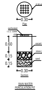
RAIN WATER PERCOLATION PIT
