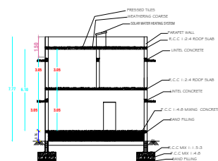
SECTION ON-"AA"
