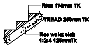
STAIR CASE
