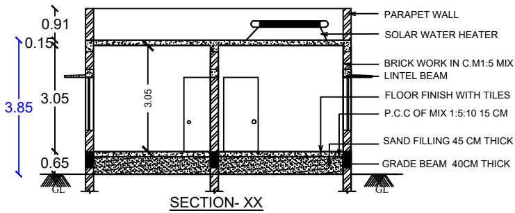
SECTION- XX
