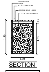
SECTION
