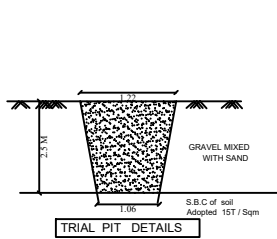
TRIAL PIT DETAILS
