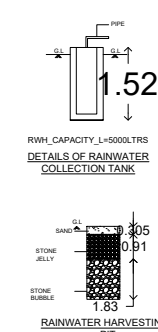
COLLECTION SUMP FOR HARVESTING FOR TERRACE
