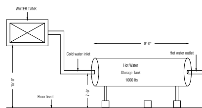
SOLAR WATER HEATER DETAILS (NOT TO SCALE)
