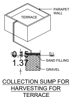
RAINWATER HARVESTING [NTS]
