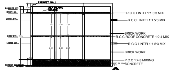
SECTION "A-B"
