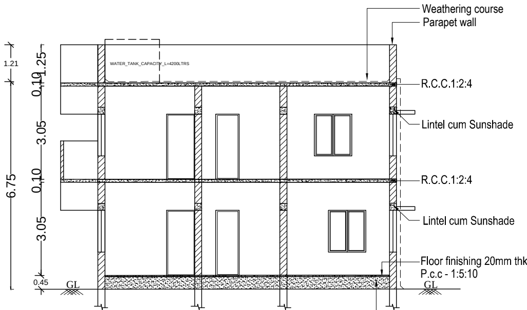
SECTION - XY
