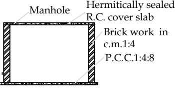
Section On 'Y-Y'
