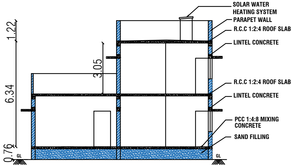
SECTION NO - "AB"
