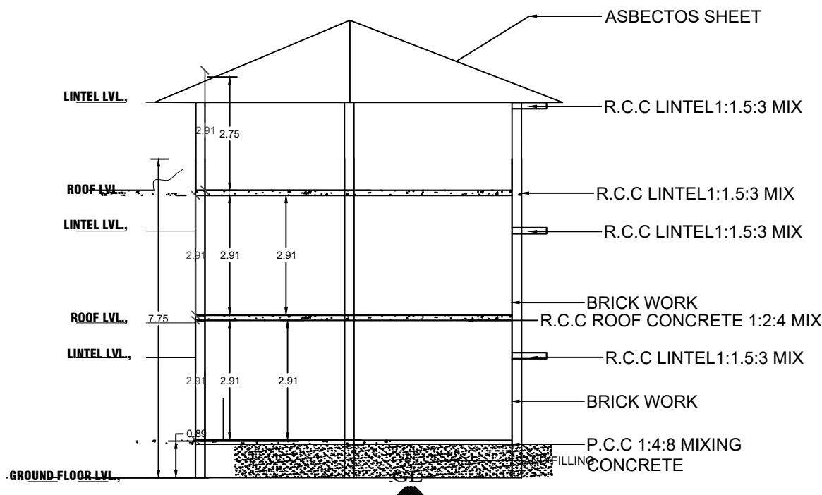
SECTION "A-B"
