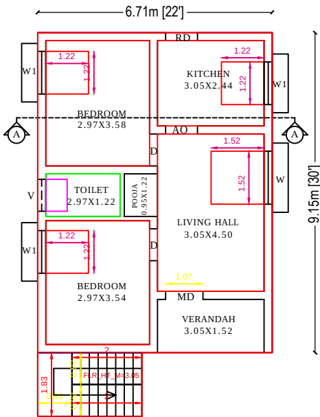
PRO.GROUND FLOOR PLAN
