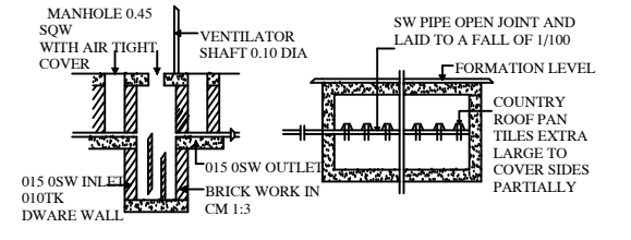
SECTION OF SEPTIC TANK
