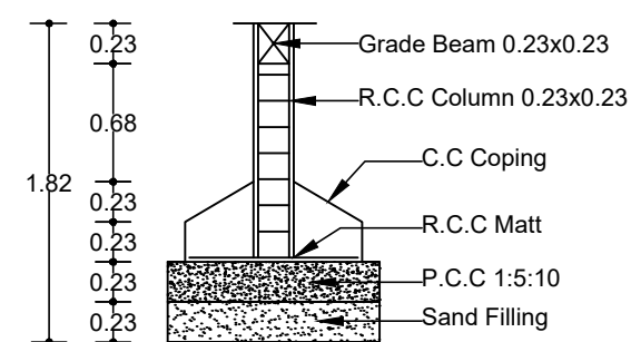
Foundation Detail
