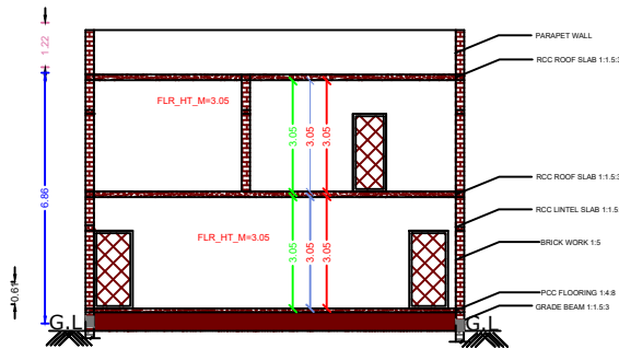
SECTION A,B
