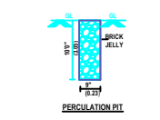
PERCOLATION PIT
