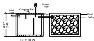
SECTION
