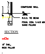
SECTION
