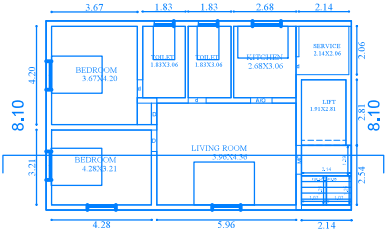
EXI-FIRST FLOOR PLAN
