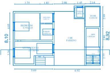
EXI-GROUND FLOOR PLAN
