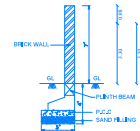
COMPOUND WALL DETAIL
