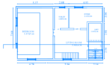
PRO-THIRD FLOOR PLAN
