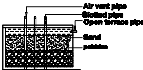
RAIN WATER COLLECTING CHAMBER
