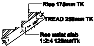
STAIR CASE
