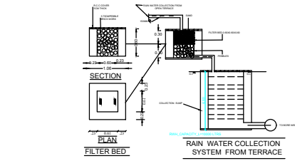
RAIN WATER HARVESTING 1. PERCOLATION PIT
