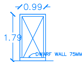
WICKET GATE
