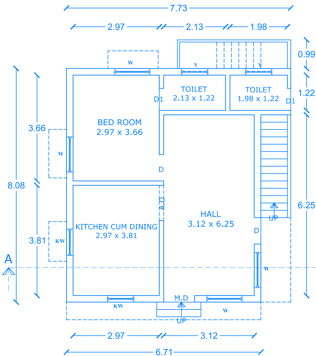
FLOOR PLAN
