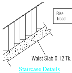
Staircase Details
