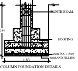
COLUMN FOUNDATION DETAILS
