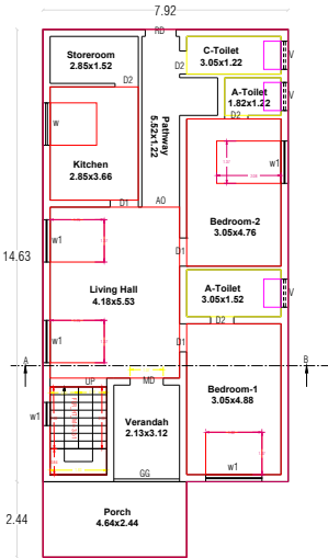
PRO GROUND FLOOR PLAN
