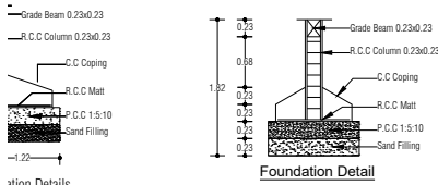
Foundation Detail
