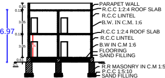
SECTION ON AB
