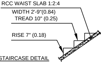
STAIRCASE DETAIL
