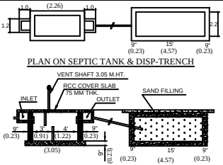
SECTION ON SEPTIC TANK & DISP-TRENCH
