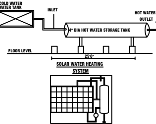
SOLAR HOT WATER SYSTEM DETAILS
