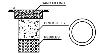
RAIN WATER HARVESTING SYSYTEM
