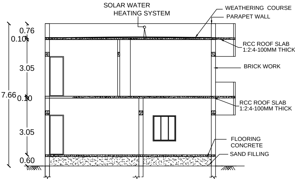
SECTION ON BR
