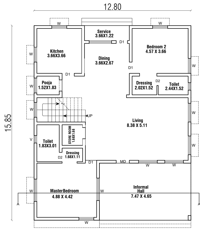
GR PLAN
