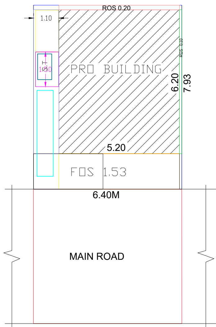
SITE PLAN
