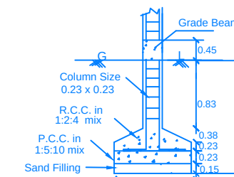
COLUMN DETAILS
