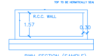
RWH_SECTION (SAMPLE)
