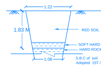
TRIAL PIT DETAILS
