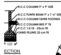
COLUMN DETAILS PLAN
