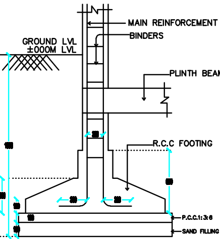
TYPICAL SECTION OF R.C.C COLUMN FOUNDATION SCALE : 1" = 2'-0" NOT TO SCALE
