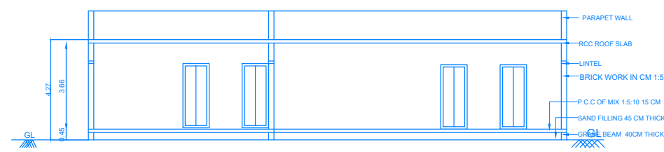
SECTION - AA1
