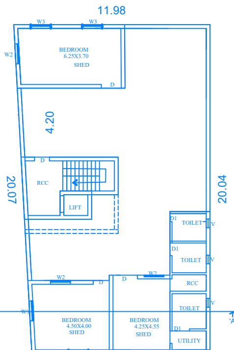
PRO.THIRD FLOOR PLAN
