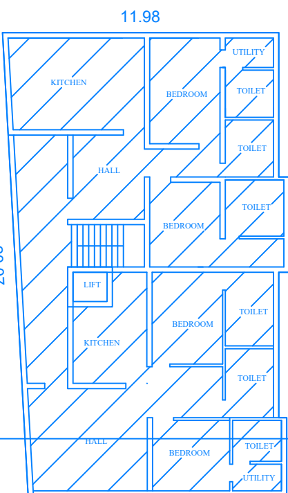
EXI.SECOND FLOOR PLAN
